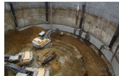
Nuclear Reactor Caisson Removal HUMBOLDT BAY, CA
